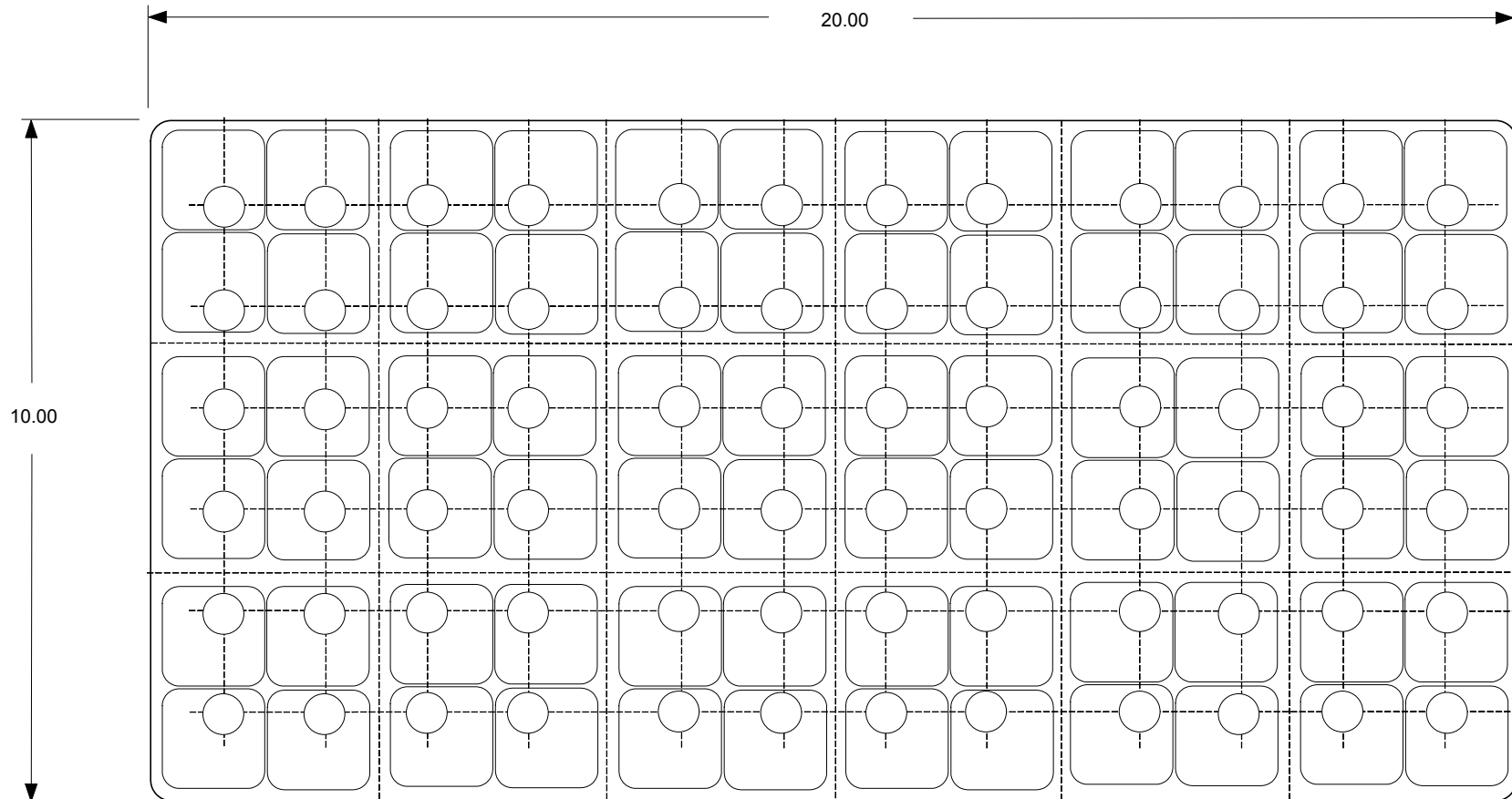
324/18-04T (10x20) Plug Positions 4/4/02 2x2 pattern, 3 rows remain in plug tray (9,18,27) Punch Plate p/n D303A0043
