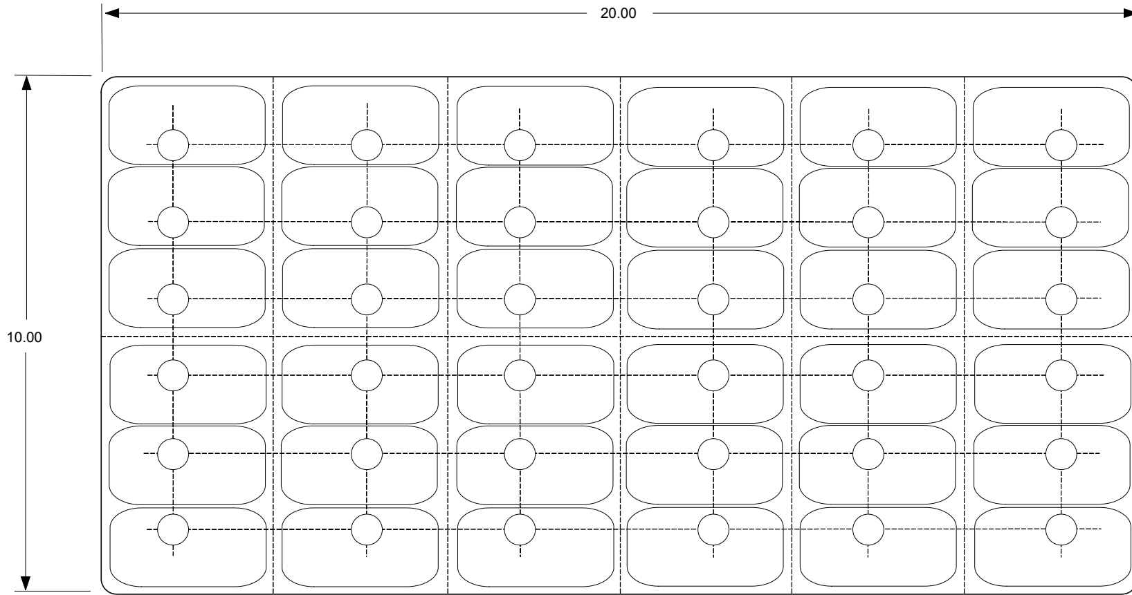
324/12-03T (10x20) Plug Positions 4/4/02 4x2 pattern, 3 rows remain in plug tray (5,14,23) Punch Plate p/n D303A0032
